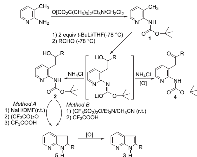
Scheme 1. Proposed synthesis of 2-substituted-7-azaindoles.
