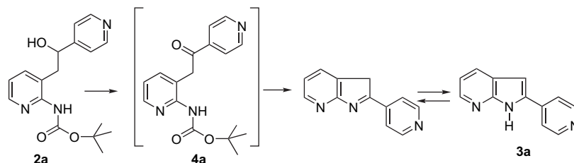
Scheme 2. Alternative synthesis of 2-substituted-7-azaindoles.
