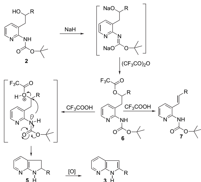
Scheme 3. Tentative mechanism for the cyclization (method A).
